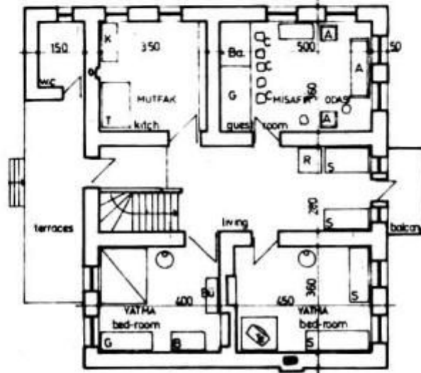
upper floor plan 1/100
