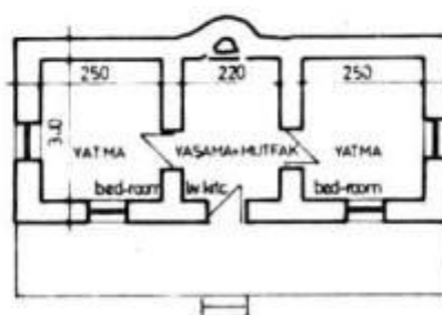
plan 1/100
